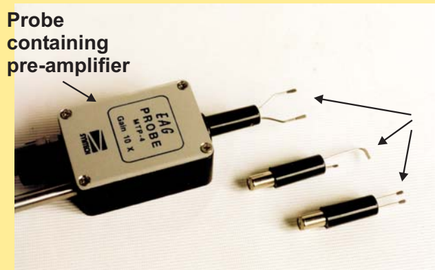
EAG Probe
